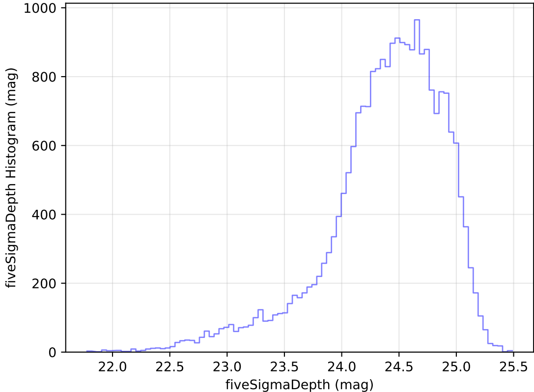
ddf_acor_sf10_lsf20_lsr20_v3.4_10yrs Yr 1 g band: fiveSigmaDepth Histogram
