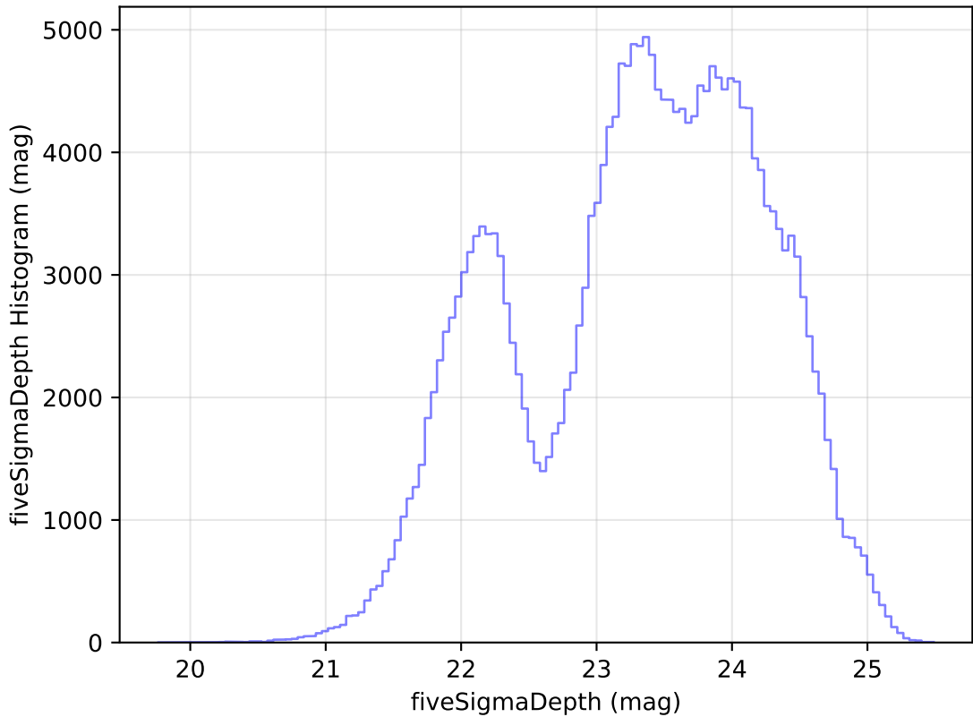
ddf_acor_sf10_lsf20_lsr20_v3.4_10yrs Yr 1 all bands: fiveSigmaDepth Histogram
