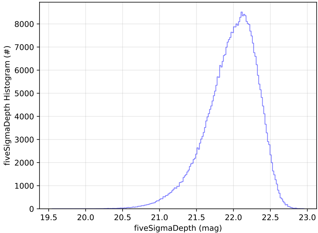
ddf_acor_sf10_lsf20_lsr20_v3.4_10yrs WFD y band: fiveSigmaDepth Histogram
