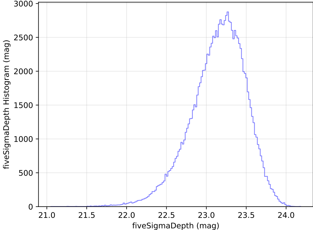
ddf_acor_sf10_lsf20_lsr20_v3.4_10yrs WFD u band: fiveSigmaDepth Histogram
