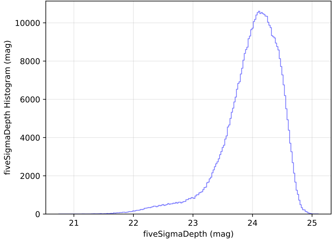
ddf_acor_sf10_lsf20_lsr20_v3.4_10yrs WFD r band: fiveSigmaDepth Histogram
