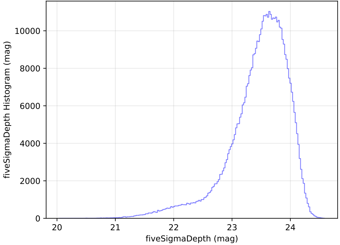
ddf_acor_sf10_lsf20_lsr20_v3.4_10yrs WFD i band: fiveSigmaDepth Histogram
