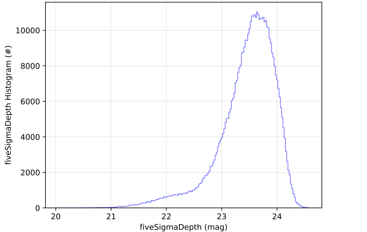
ddf_acor_sf10_lsf20_lsr20_v3.4_10yrs WFD i band: fiveSigmaDepth Histogram
