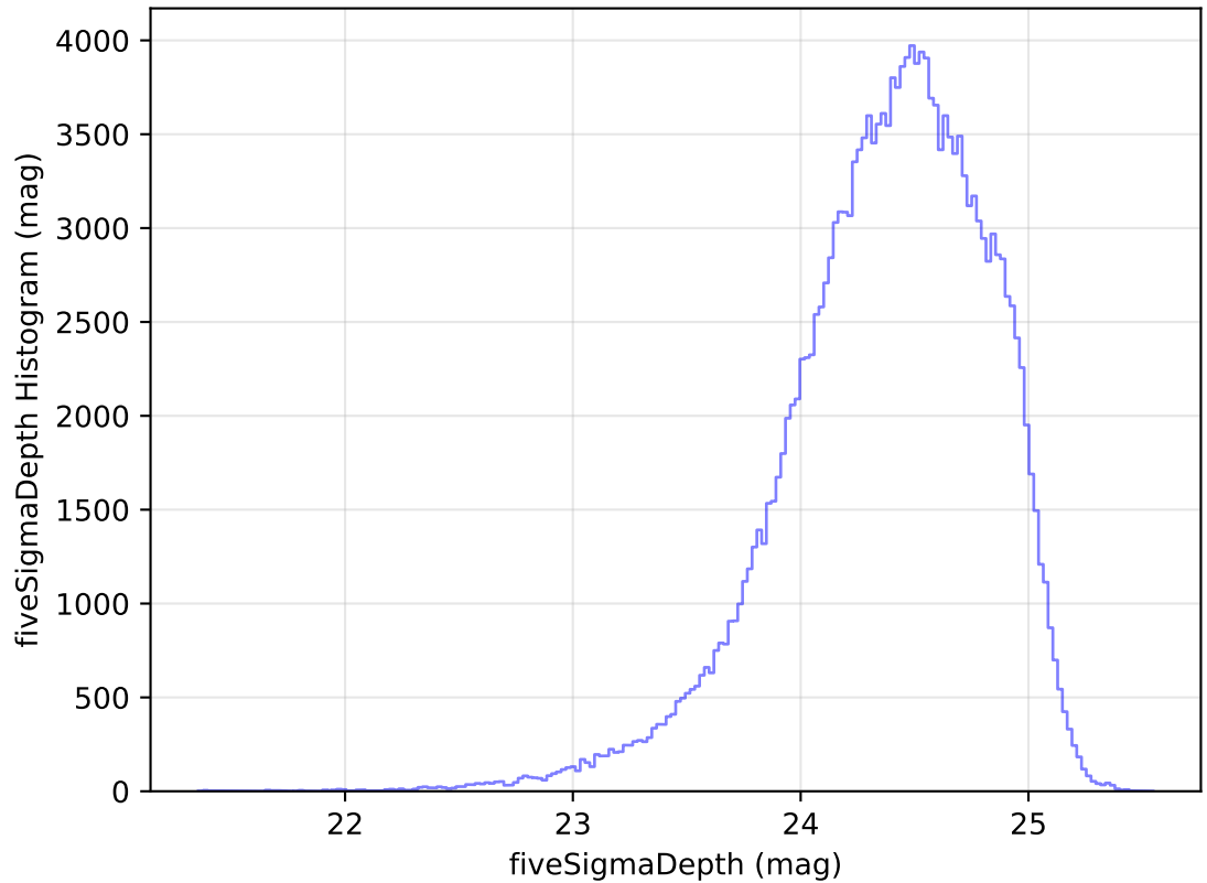
ddf_acor_sf10_lsf20_lsr20_v3.4_10yrs WFD g band: fiveSigmaDepth Histogram
