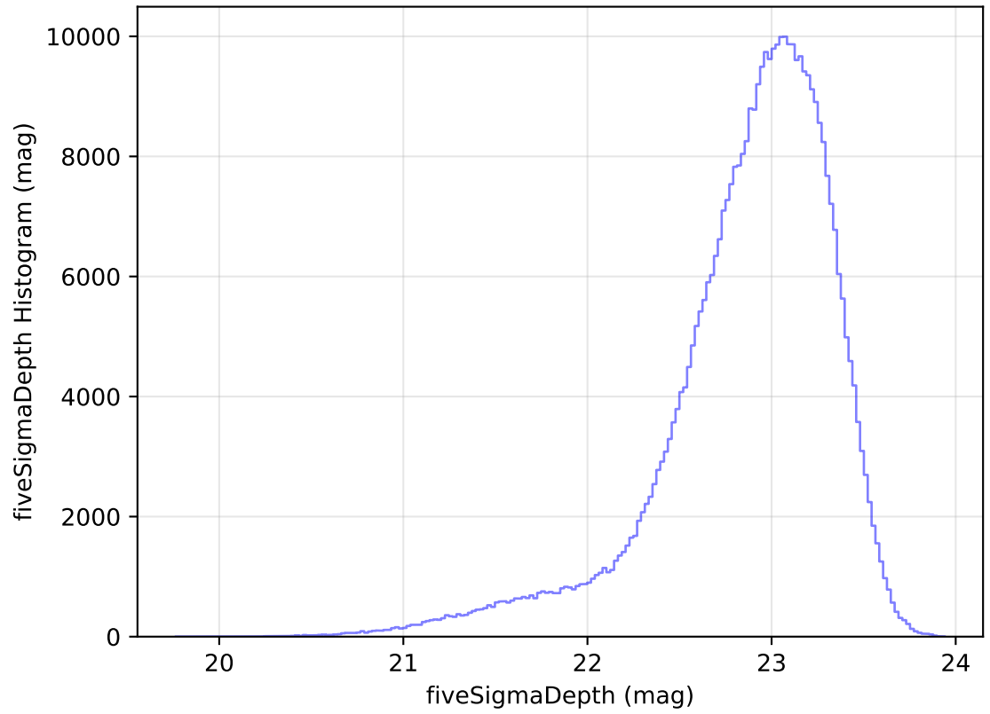
ddf_acor_sf10_lsf20_lsr20_v3.4_10yrs All sky z band: fiveSigmaDepth Histogram
