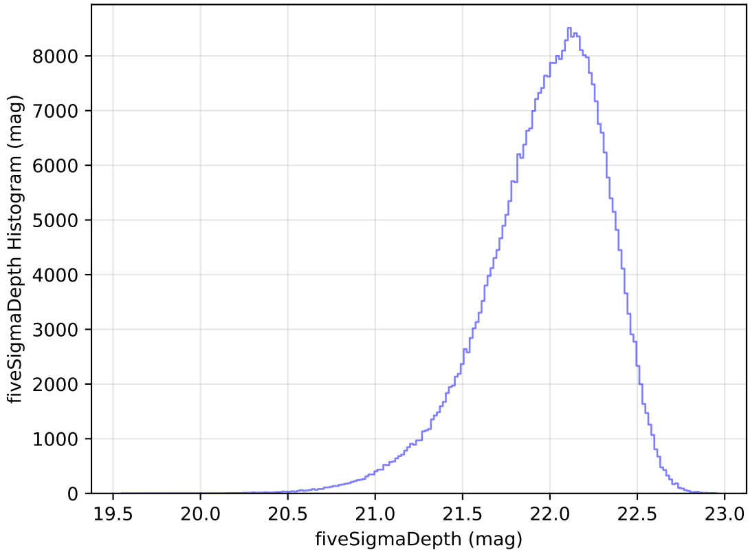
ddf_acor_sf10_lsf20_lsr20_v3.4_10yrs All sky y band: fiveSigmaDepth Histogram
