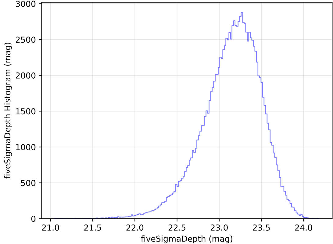
ddf_acor_sf10_lsf20_lsr20_v3.4_10yrs All sky u band: fiveSigmaDepth Histogram
