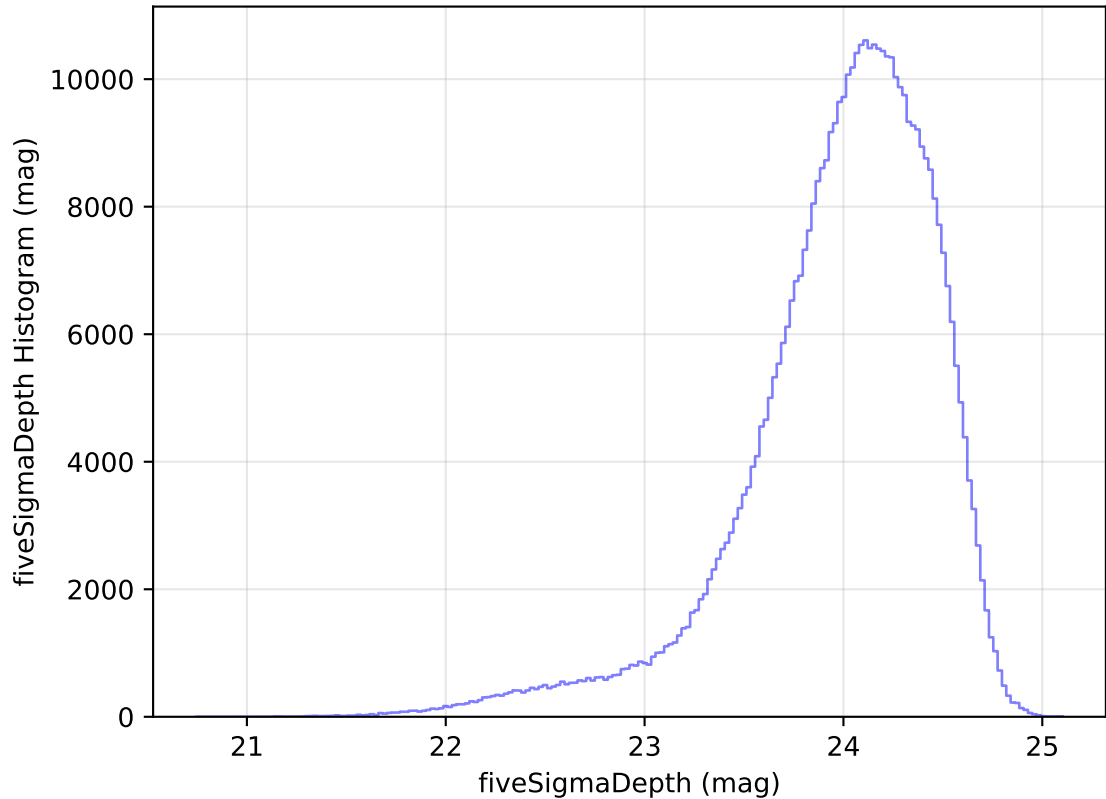
ddf_acor_sf10_lsf20_lsr20_v3.4_10yrs All sky r band: fiveSigmaDepth Histogram
