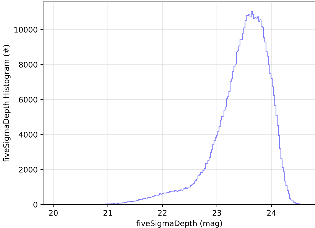
ddf_acor_sf10_lsf20_lsr20_v3.4_10yrs All sky i band: fiveSigmaDepth Histogram
