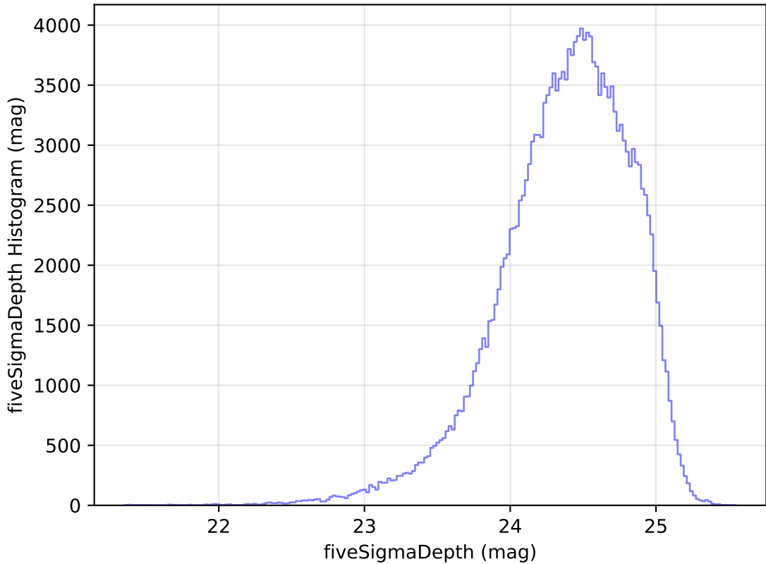
ddf_acor_sf10_lsf20_lsr20_v3.4_10yrs All sky g band: fiveSigmaDepth Histogram
