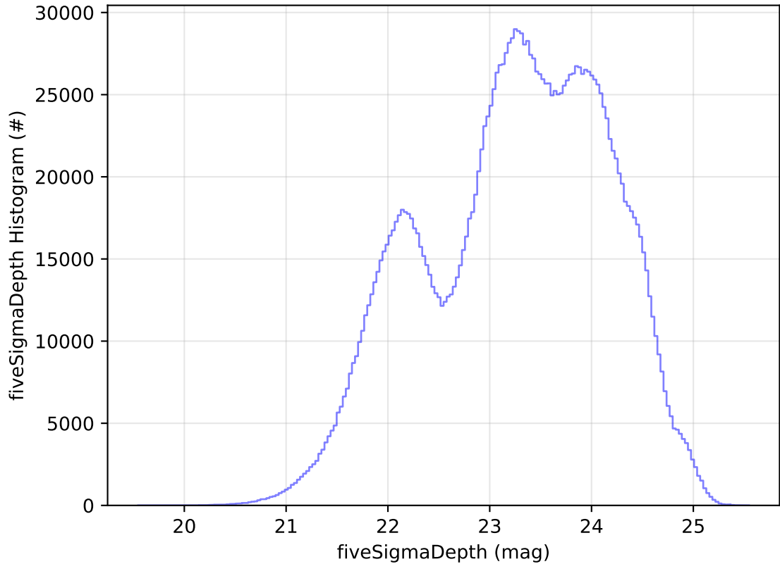
ddf_acor_sf10_lsf20_lsr20_v3.4_10yrs All sky all bands: fiveSigmaDepth Histogram
