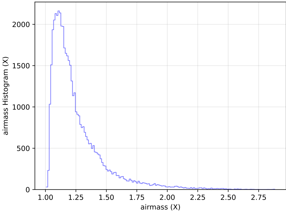
ddf_acor_sf10_ls20_lsr20_v3.4_10yrs Yr 1 y band: airmass Histogram
