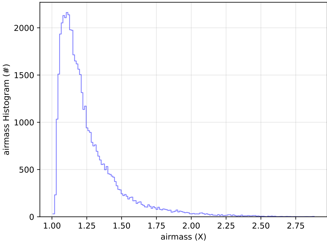
ddf_acor_sf10_lsf20_lsr20_v3.4_10yrs Yr 1 y band: airmass Histogram
