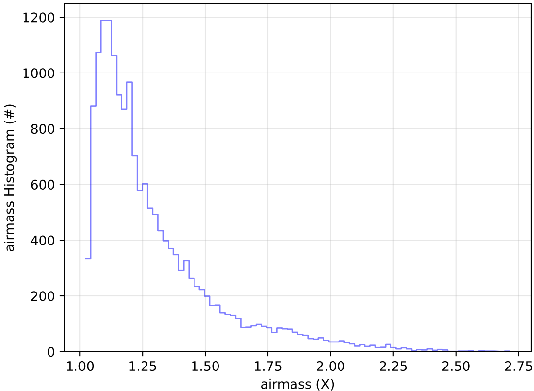
ddf_acor_sf10_lsf20_lsr20_v3.4_10yrs Yr 1 u band: airmass Histogram
