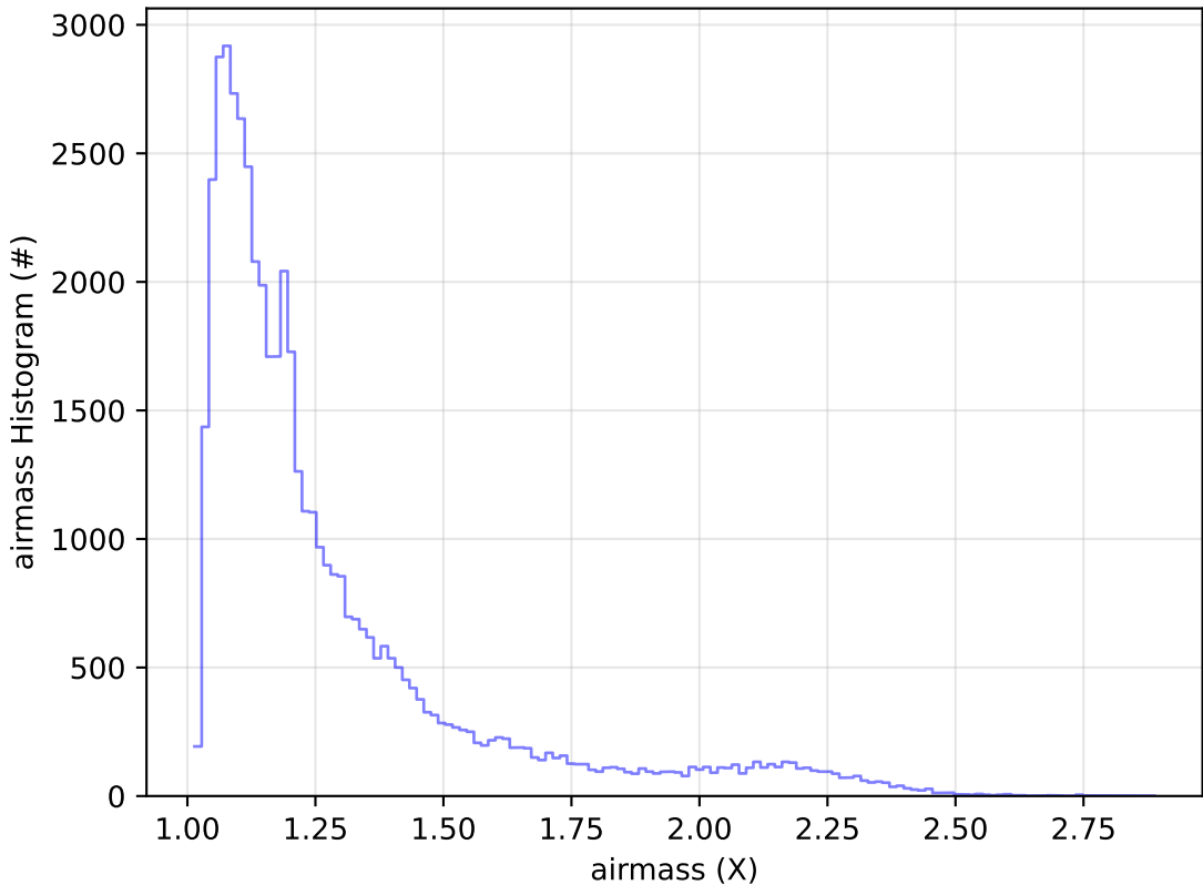
ddf_acor_sf10_lsf20_lsr20_v3.4_10yrs Yr 1 r band: airmass Histogram
