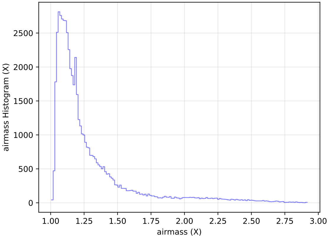
ddf_acor_sf10_lsf20_lsr20_v3.4_10yrs Yr 1 i band: airmass Histogram
