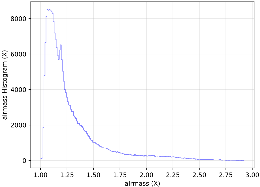
ddf_acor_sf10_lsf20_lsr20_v3.4_10yrs Yr 1 all bands: airmass Histogram
