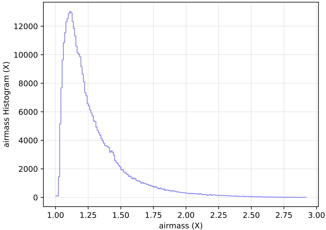
ddf_acor_sf10_lsf20_lsr20_v3.4_10yrs WFD y band: airmass Histogram
