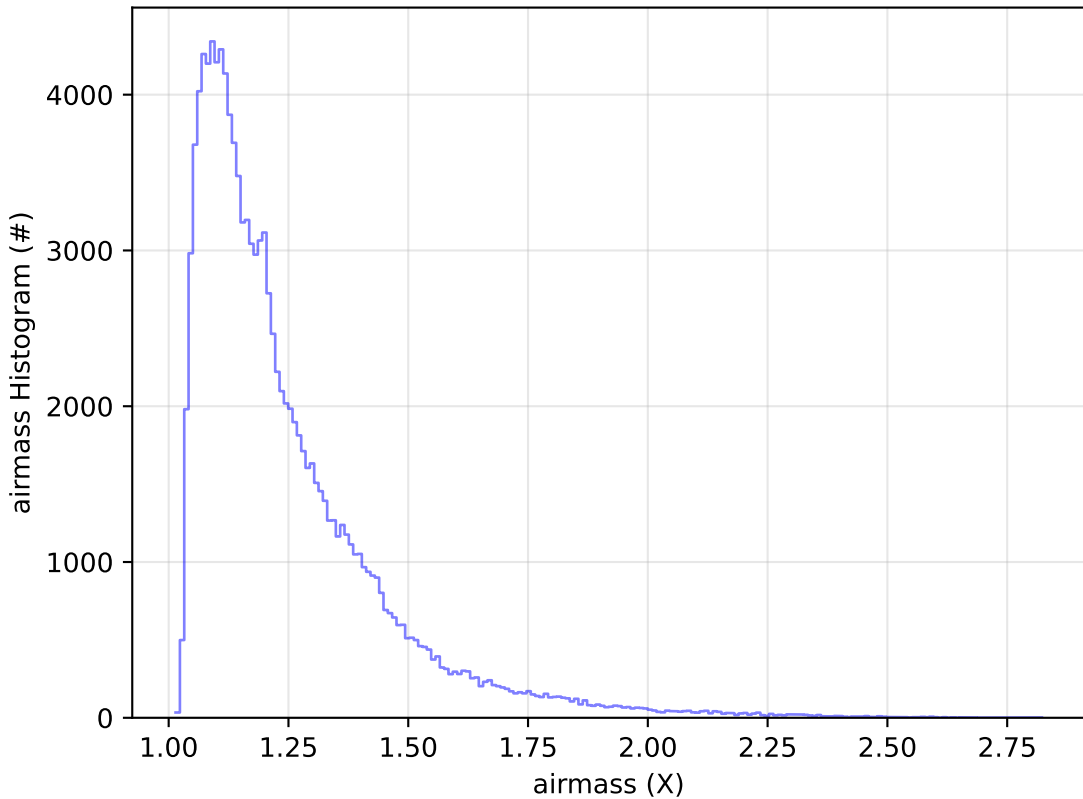
ddf_acor_sf10_lsf20_lsr20_v3.4_10yrs WFD u band: airmass Histogram
