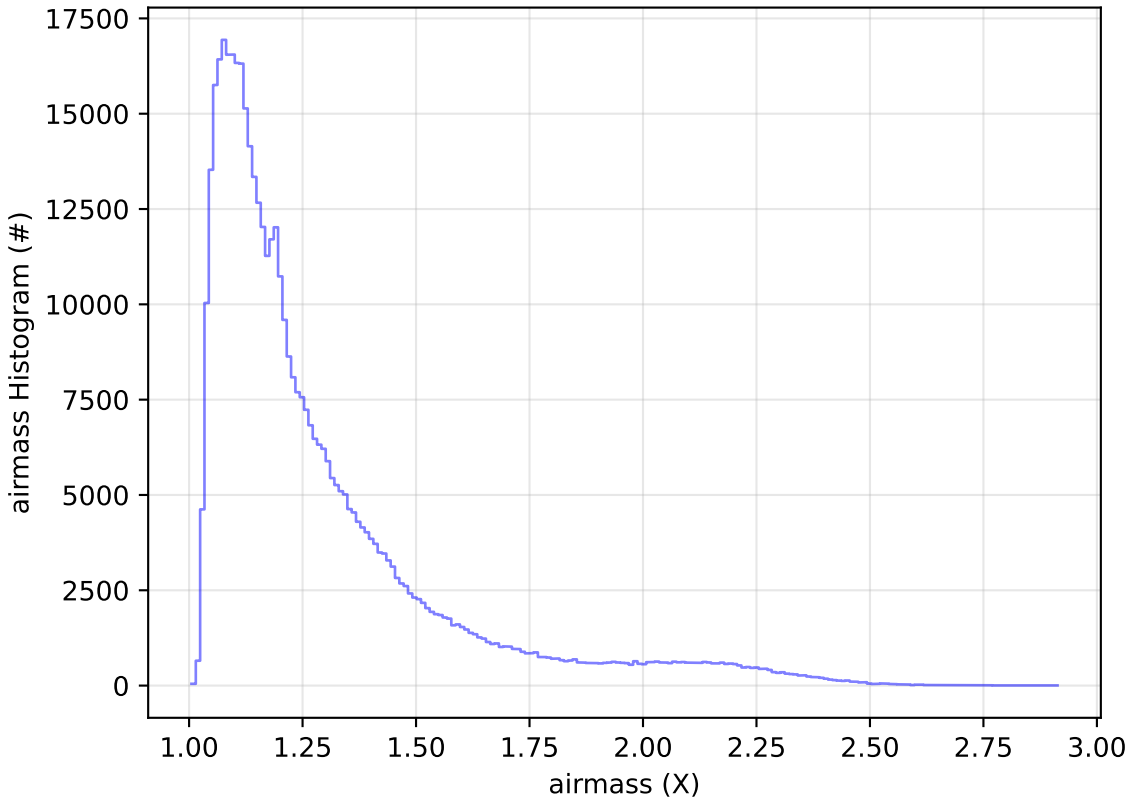
ddf_acor_sf10_lsf20_lsr20_v3.4_10yrs WFD r band: airmass Histogram
