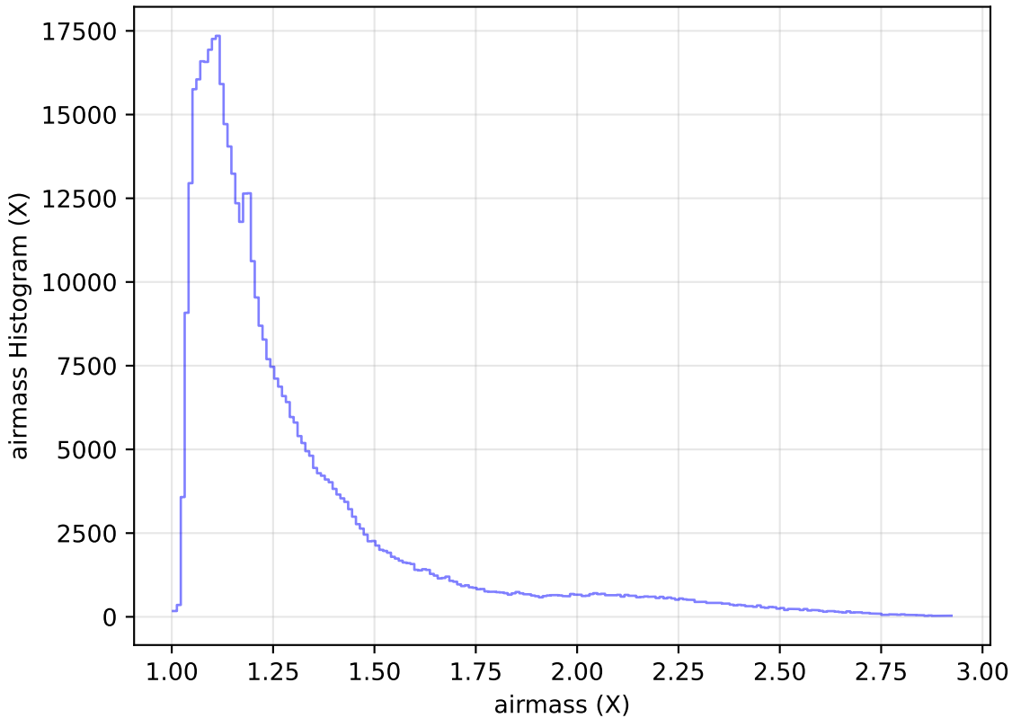
ddf_acor_sf10_lsf20_lsr20_v3.4_10yrs WFD i band: airmass Histogram
