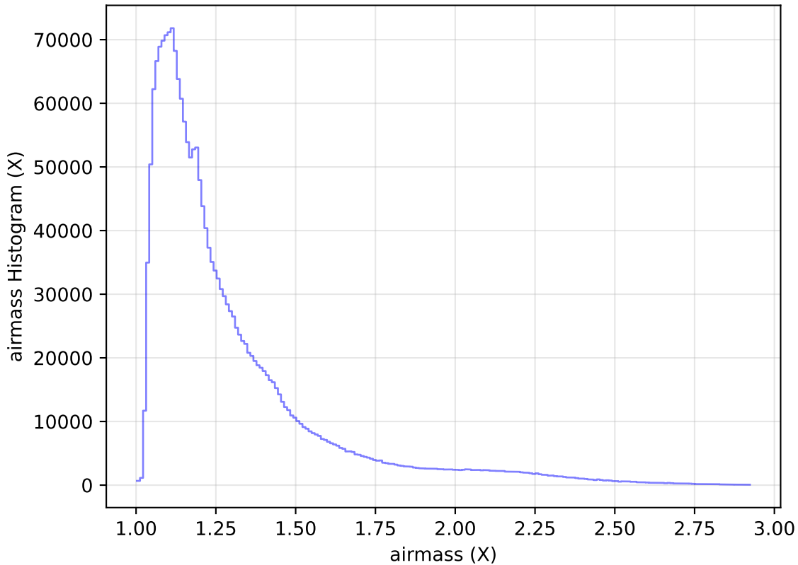
ddf_acor_sf10_lsf20_lsr20_v3.4_10yrs WFD all bands: airmass Histogram
