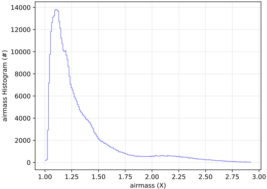
ddf_acor_sf10_lsf20_lsr20_v3.4_10yrs All sky z band: airmass Histogram
