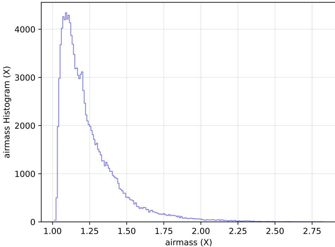
ddf_acor_sf10_lsf20_lsr20_v3.4_10yrs All sky u band: airmass Histogram
