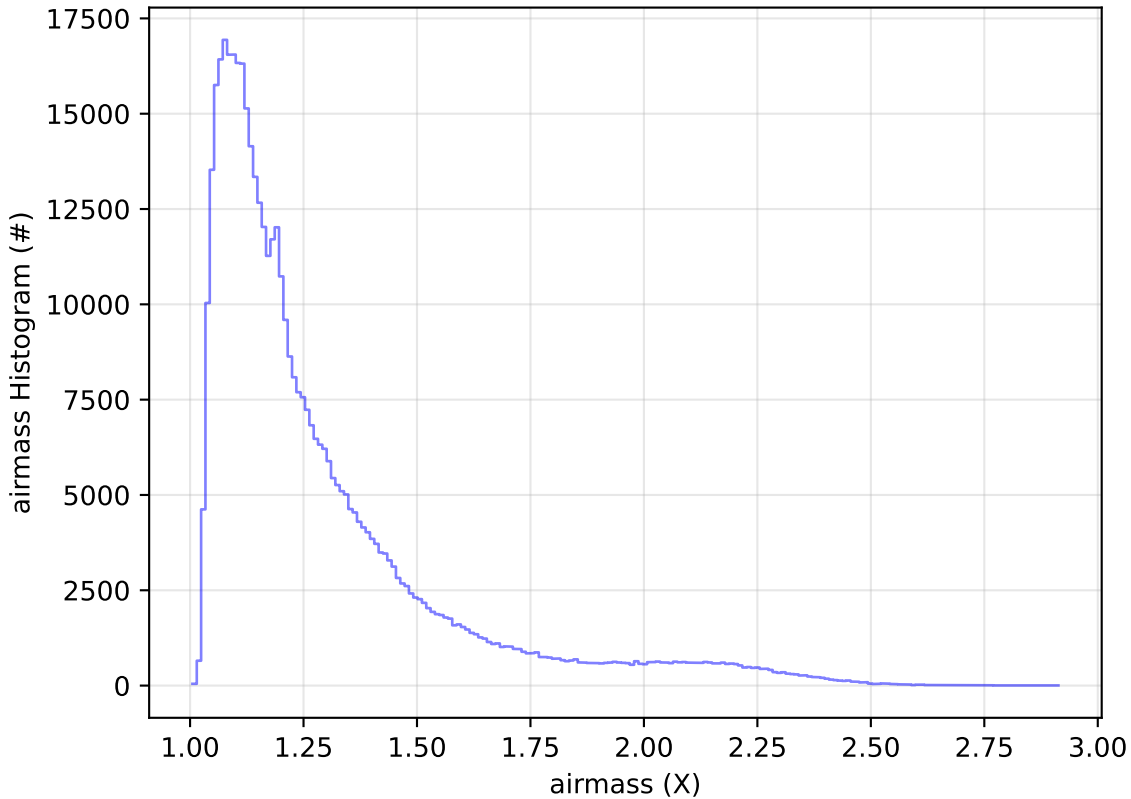
ddf_acor_sf10_lsf20_lsr20_v3.4_10yrs All sky r band: airmass Histogram
