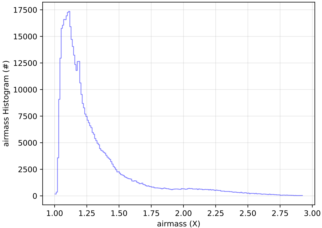
ddf_acor_sf10_lsf20_lsr20_v3.4_10yrs All sky i band: airmass Histogram
