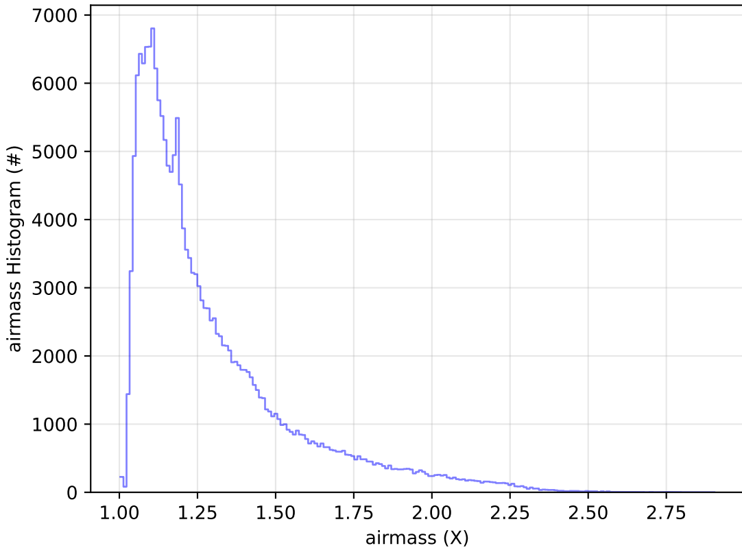
ddf_acor_sf10_lsf20_lsr20_v3.4_10yrs All sky g band: airmass Histogram
