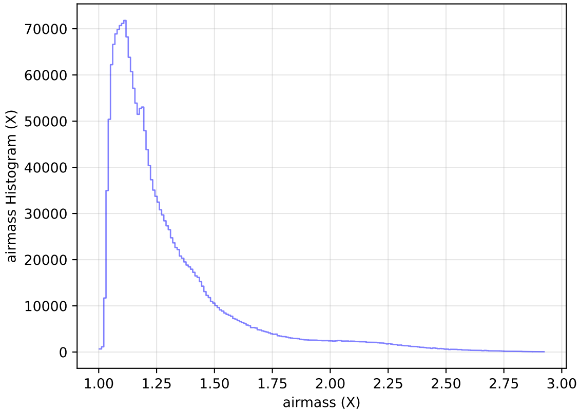
ddf_acor_sf10_lsf20_lsr20_v3.4_10yrs All sky all bands: airmass Histogram
