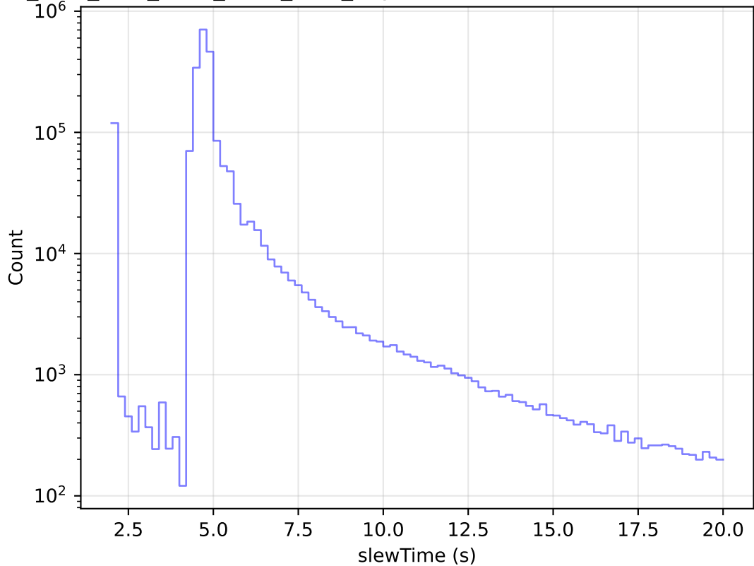
ddf_acor_sf10_Isf20_Isr20_v3.4_10yrs All visits: Zoom Slew Time Histogram
