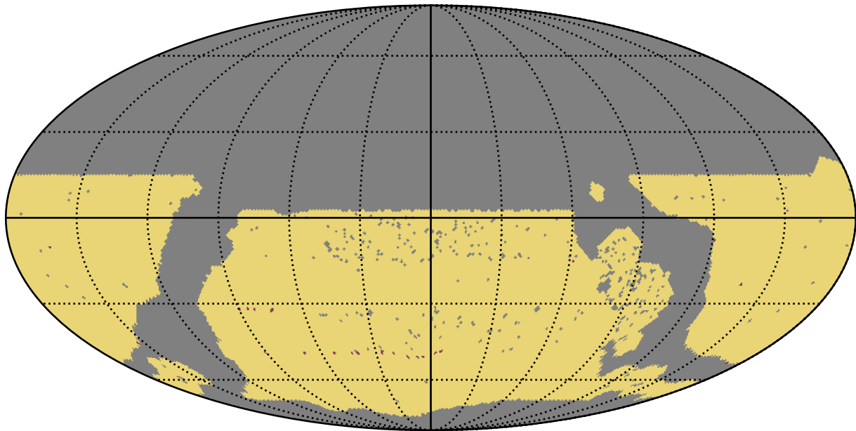
ddf_acor_sf10_lsf20_lsr20_v3.4_10yrs WFD: RapidRevisits
