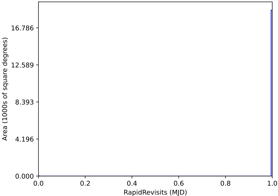
ddf_acor_sf10_lsf20_lsr20_v3.4_10yrs WFD: RapidRevisits
