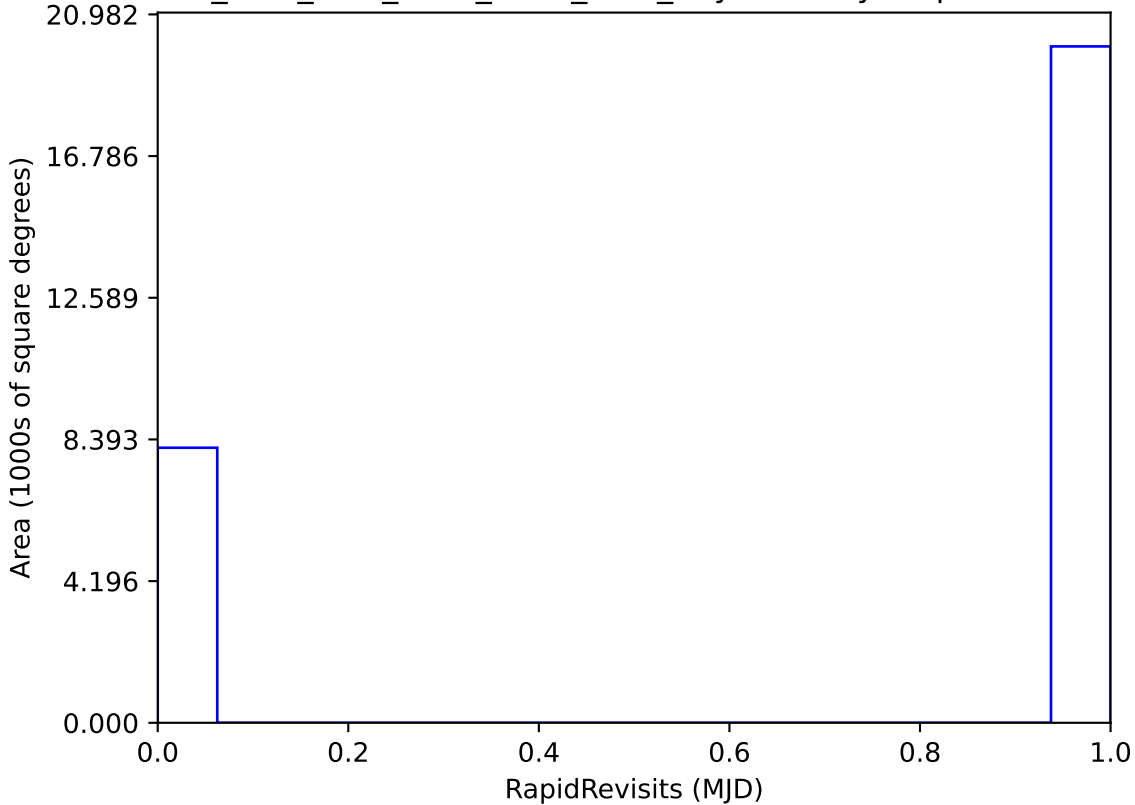
ddf_acor_sf10_lsf20_lsr20_v3.4_10yrs All sky: RapidRevisits
