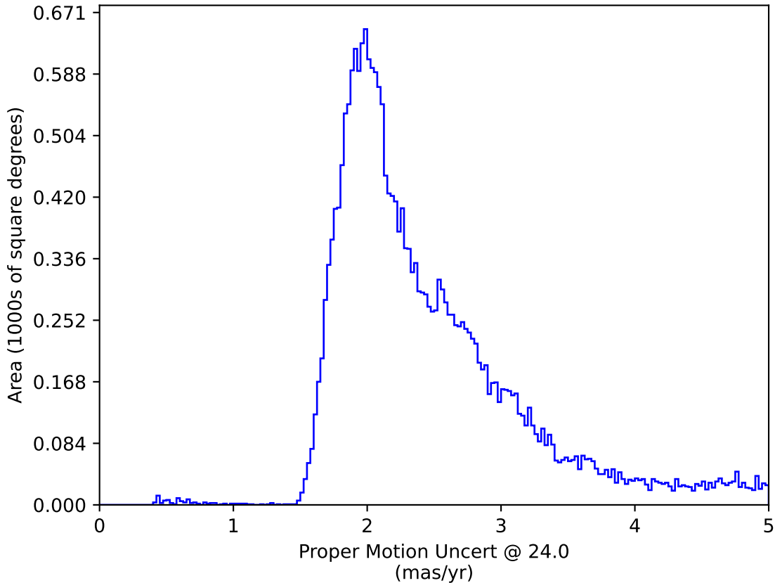
ddf_acor_sf10_lsf20_lsr20_v3.4_10yrs All sky: Proper Motion Uncert @ 24.0
