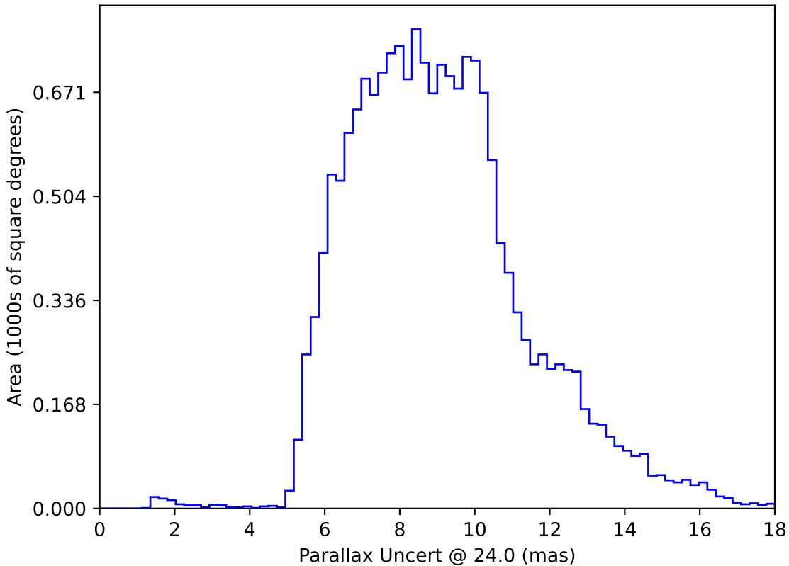
ddf_acor_sf10_lsf20_lsr20_v3.4_10yrs WFD: Parallax Uncert @ 24.0
