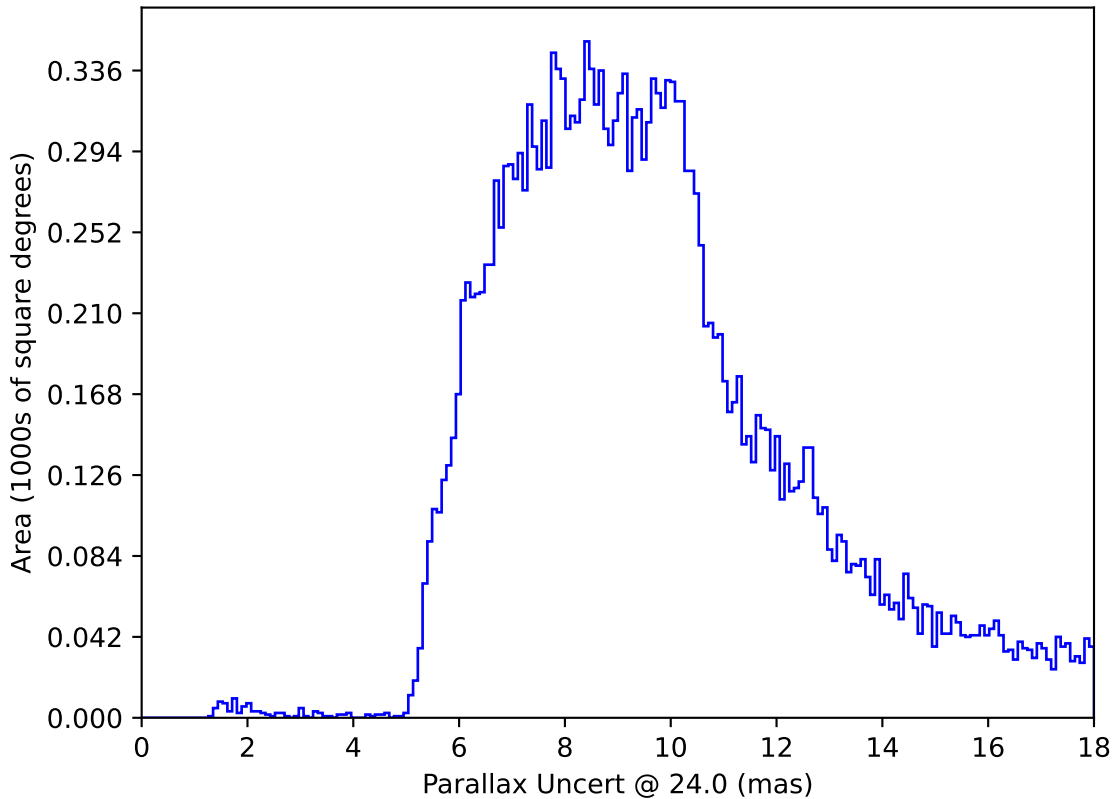
ddf_acor_sf10_lsf20_lsr20_v3.4_10yrs All sky: Parallax Uncert @ 24.0
