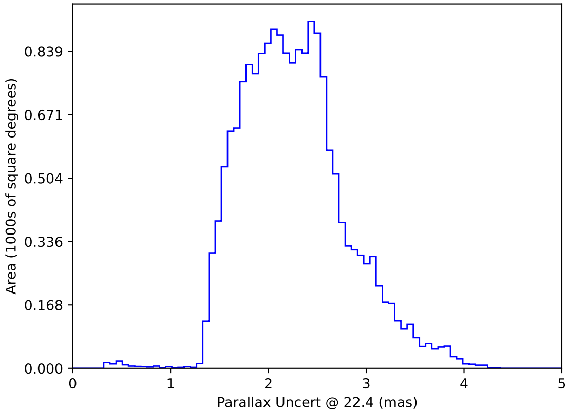
ddf_acor_sf10_lsf20_lsr20_v3.4_10yrs WFD: Parallax Uncert @ 22.4
