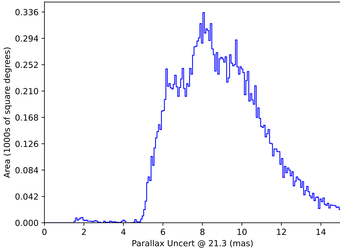
ddf_acor_sf10_lsf20_lsr20_v3.4_10yrs All sky y band only: Parallax Uncert @ 21.3
