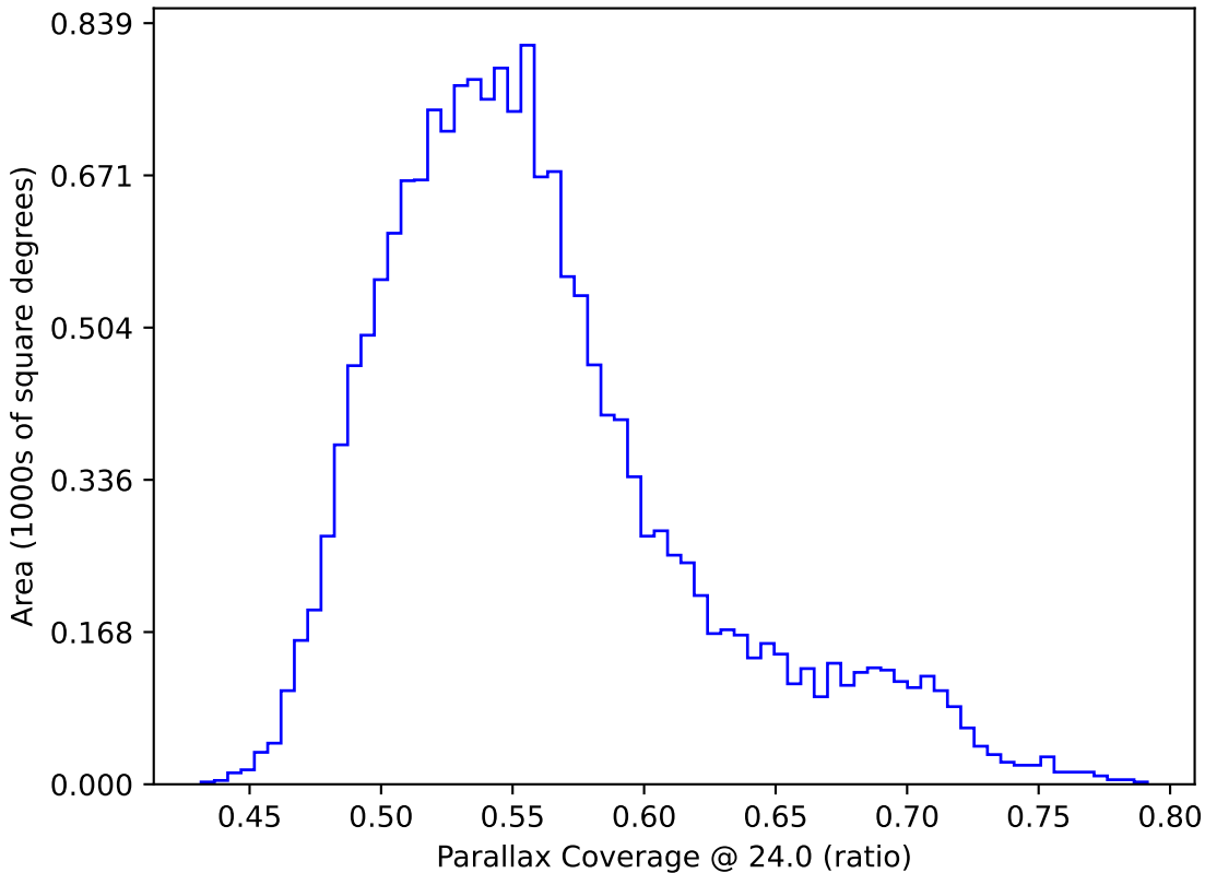
ddf_acor_sf10_lsf20_lsr20_v3.4_10yrs WFD: Parallax Coverage @ 24.0
