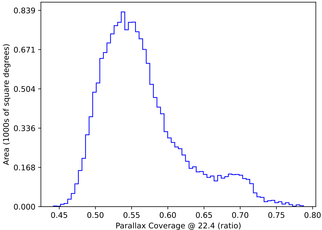
ddf_acor_sf10_lsf20_lsr20_v3.4_10yrs WFD: Parallax Coverage @ 22.4
