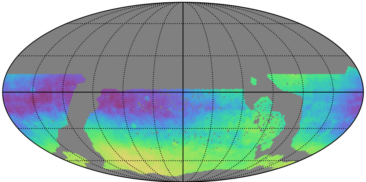
ddf_acor_sf10_lsf20_lsr20_v3.4_10yrs WFD: Parallax-DCR degeneracy @ 24.0
