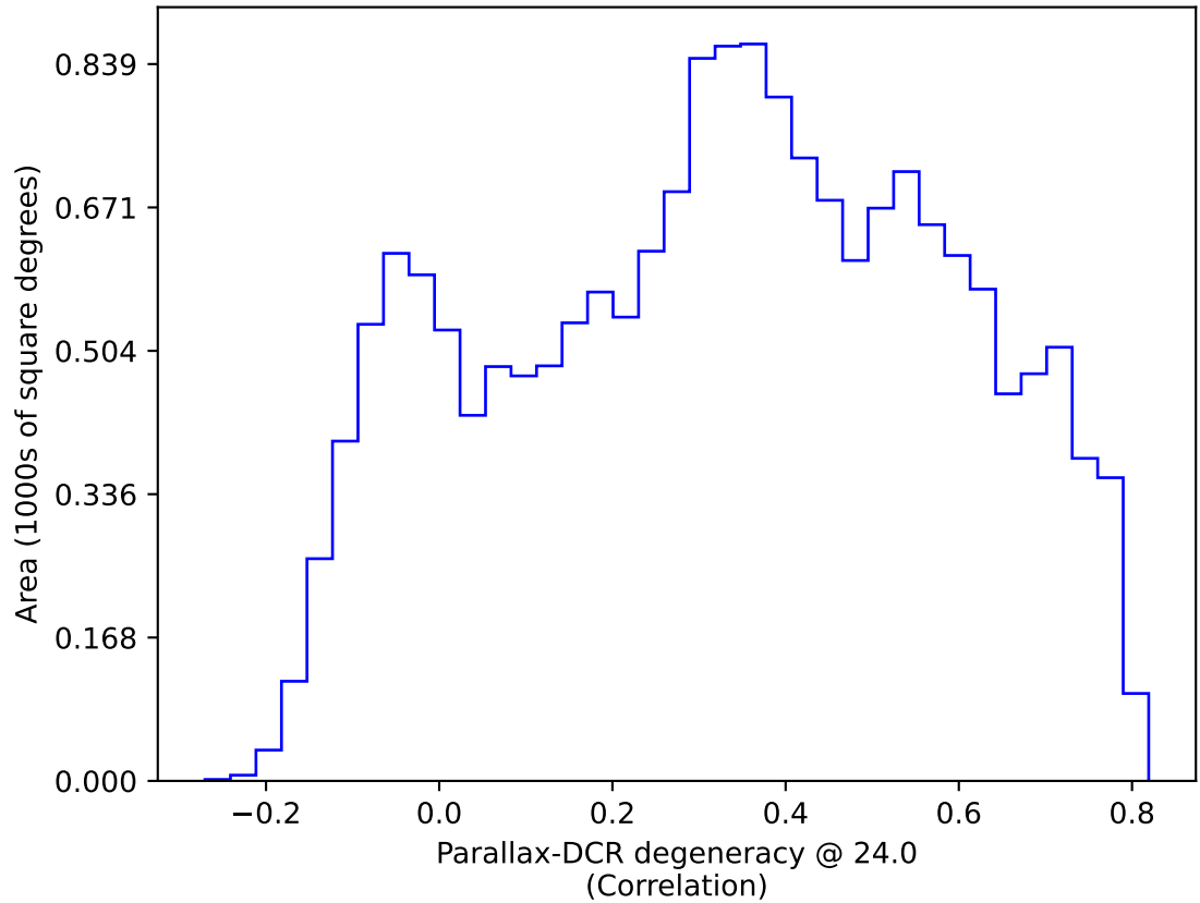
ddf_acor_sf10_lsf20_lsr20_v3.4_10yrs WFD: Parallax-DCR degeneracy @ 24.0
