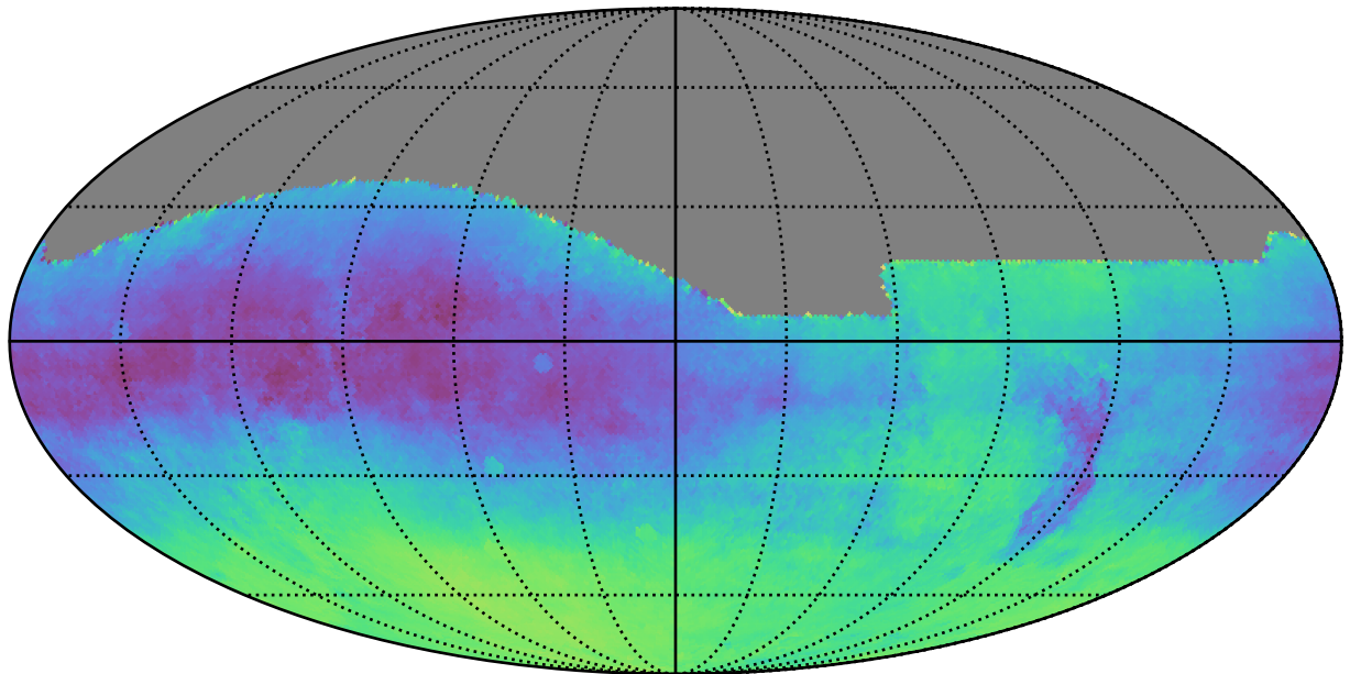
ddf_acor_sf10_lsf20_lsr20_v3.4_10yrs All sky: Parallax-DCR degeneracy @ 24.0
