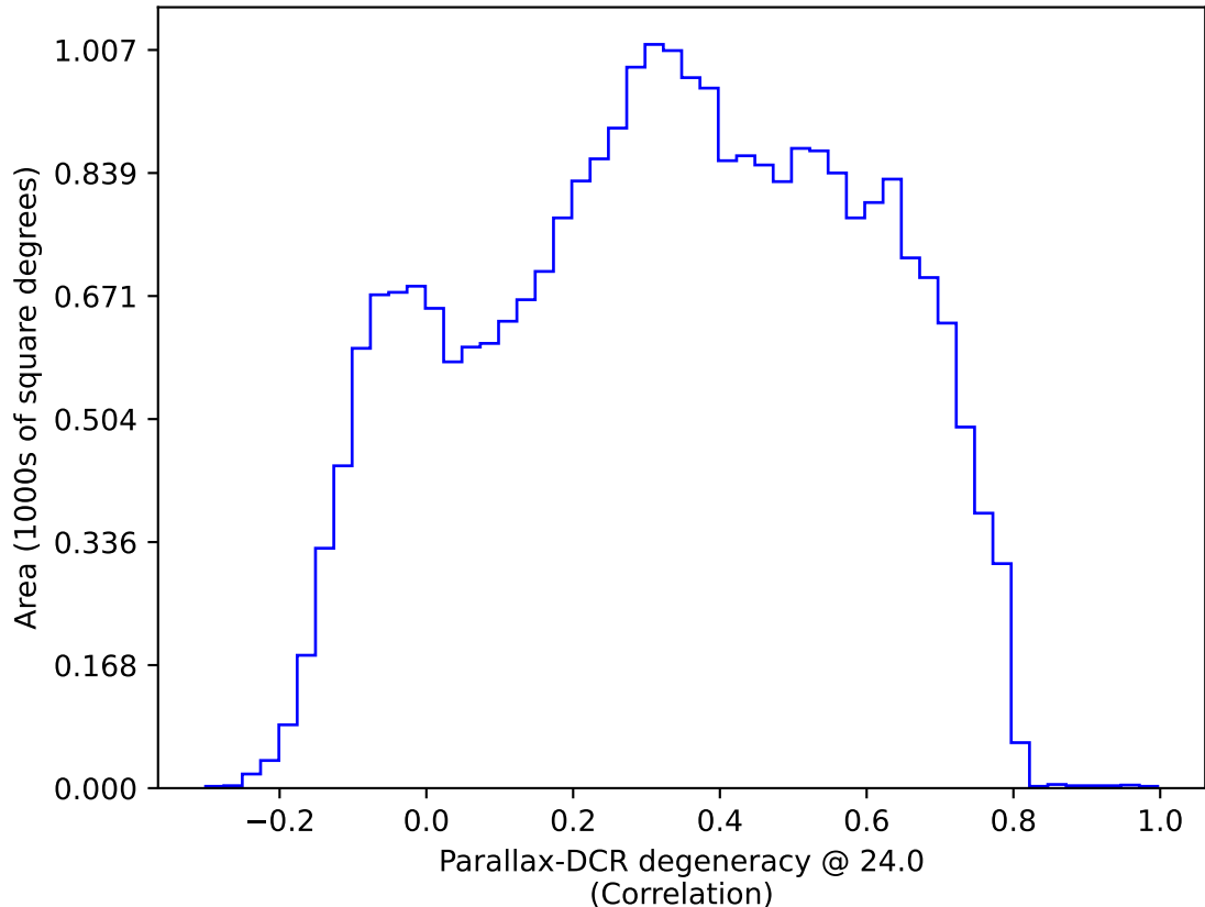
ddf_acor_sf10_ls20_lsr20_v3.4_10yrs All sky: Parallax-DCR degeneracy @ 24.0
