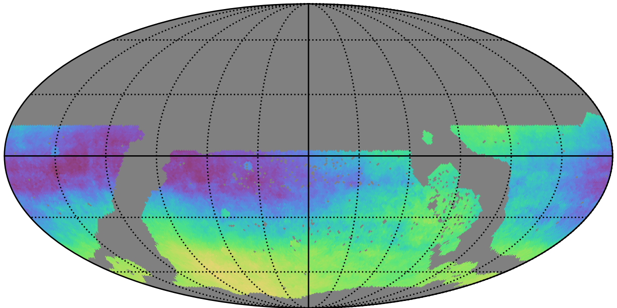
ddf_acor_sf10_lsf20_lsr20_v3.4_10yrs WFD: Parallax-DCR degeneracy @ 22.4
