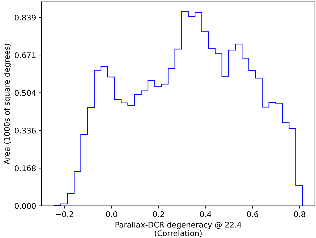
ddf_acor_sf10_lsf20_lsr20_v3.4_10yrs WFD: Parallax-DCR degeneracy @ 22.4
