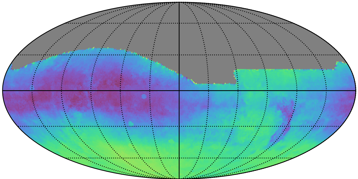
ddf_acor_sf10_lsf20_lsr20_v3.4_10yrs All sky: Parallax-DCR degeneracy @ 22.4
