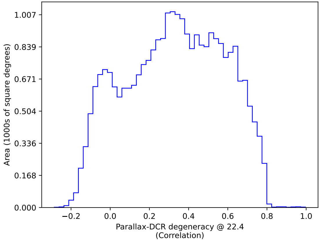
ddf_acor_sf10_lsf20_lsr20_v3.4_10yrs All sky: Parallax-DCR degeneracy @ 22.4
