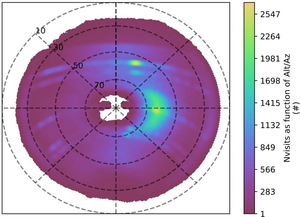
ddf_acor_sf10_lsf20_lsr20_v3.4_10yrs z band: Nvisits as function of Alt/Az
